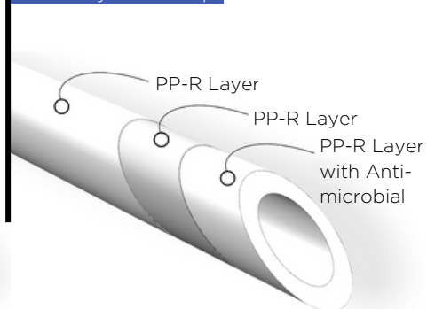
Multi-Layer PP-R Pipe
