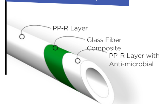
Glass Fiber Reinforced Composite
