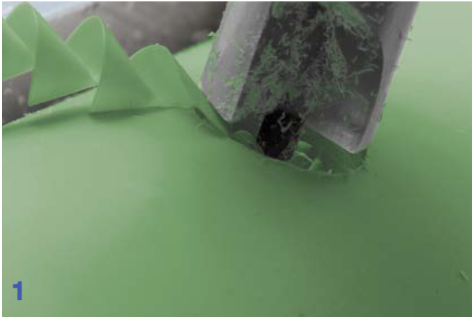
1. Drilling a hole under the pipe saddle fitting.
