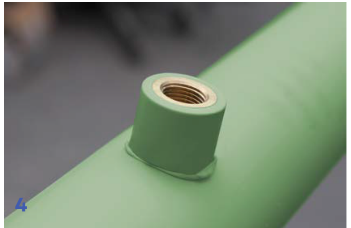
4. Ready connection. (Available in 40mm to 315mm)
